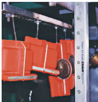
A Model 110018 18" (457mm) Super Air Knife cools molded plastic following dip molding.
